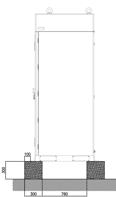
load-bearing surface
