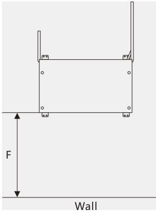
Installation clearance drawing (Vertical view)
