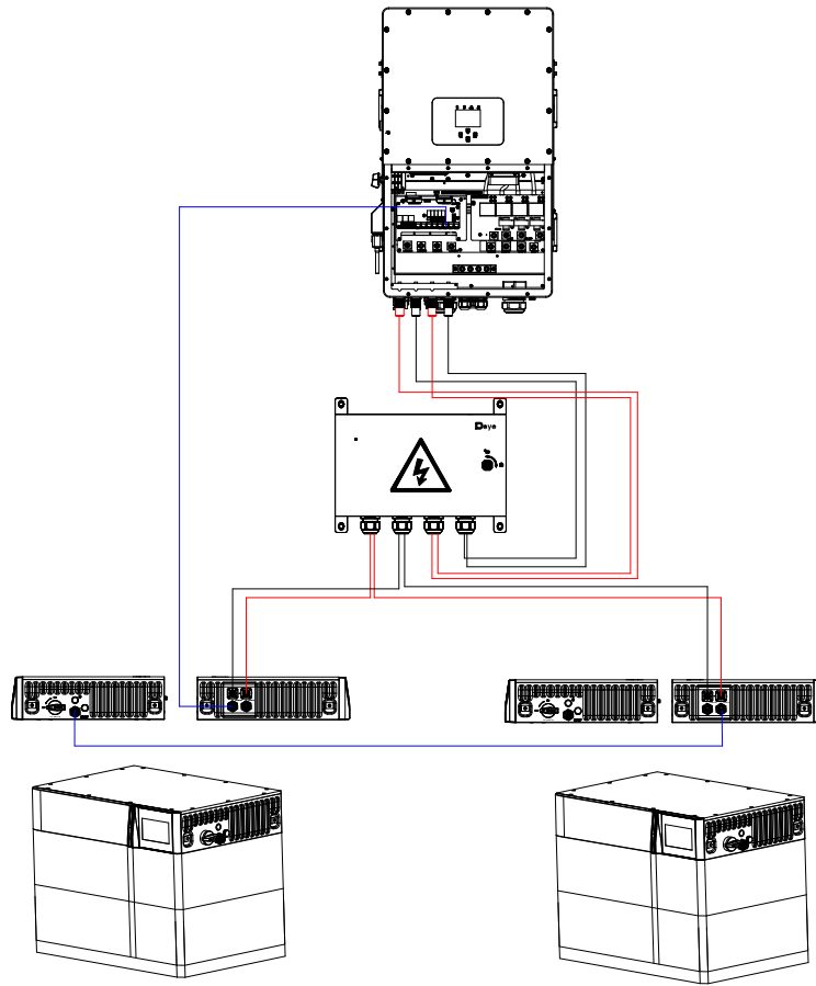
Figure 4 Cluster and cluster capacity extension wiring diagram
