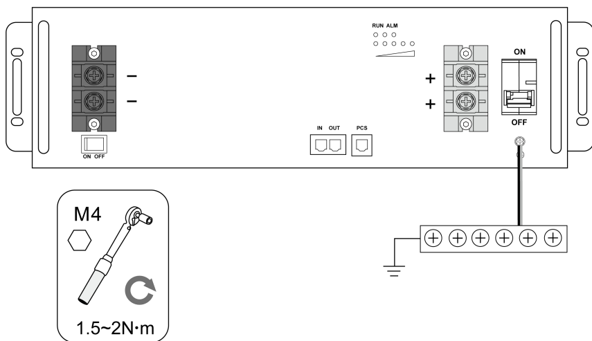
Figure 5-1: Install the Grounding Wire
