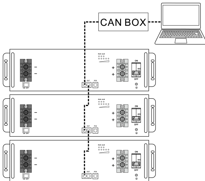
Figure 5-3: Communication Cable Connections between Battery and Computer
