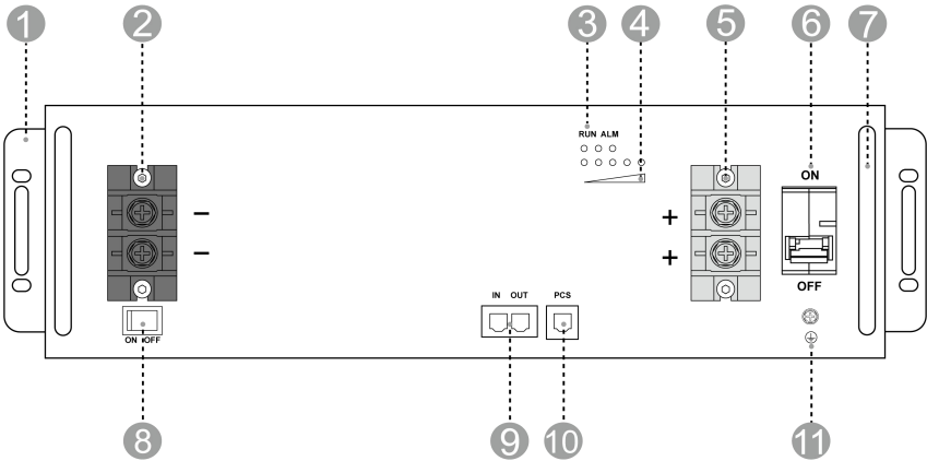
Figure 2-1: Front Panel Function Introduction
