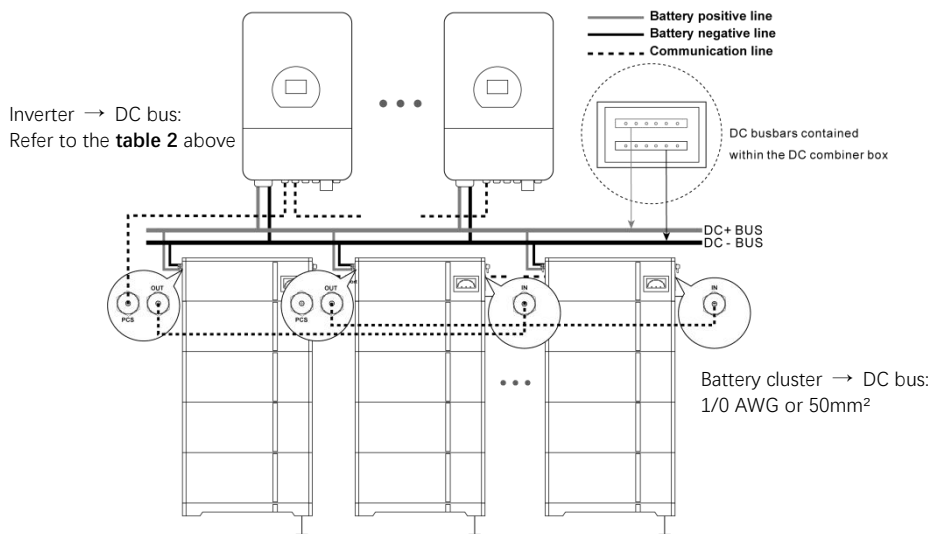
Schematic diagram of connection of multiple inverters and battery systems:
