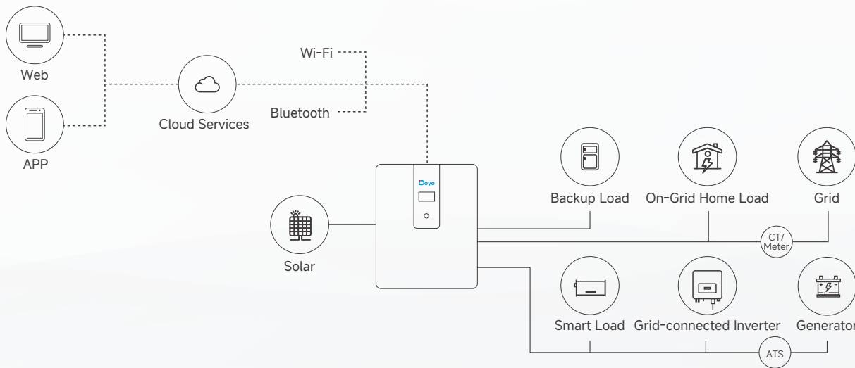
System Application Topology Diagram
